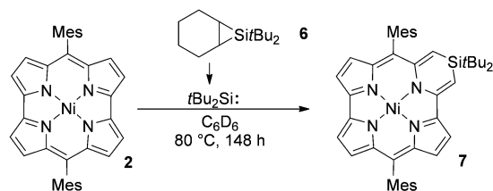
Scheme 3. Silylene transfer from silacyclopropane 6 to norcorrole 2 .
